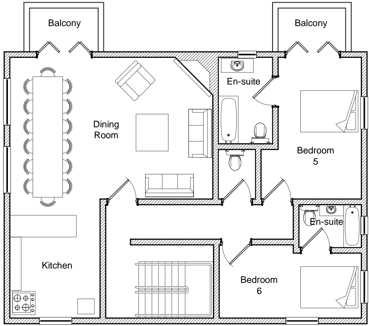
Second Floor Layout
